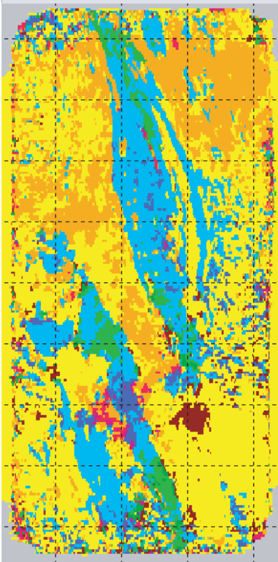
Figure 3. Fast S-wave polarization direction (degrees) and percent S-wave anisotropy from the Gessoso layer above the top-Paleocene target at the Emilio field. Note the distinct influence of northwest-southeast trending faults and compartmentalization.
