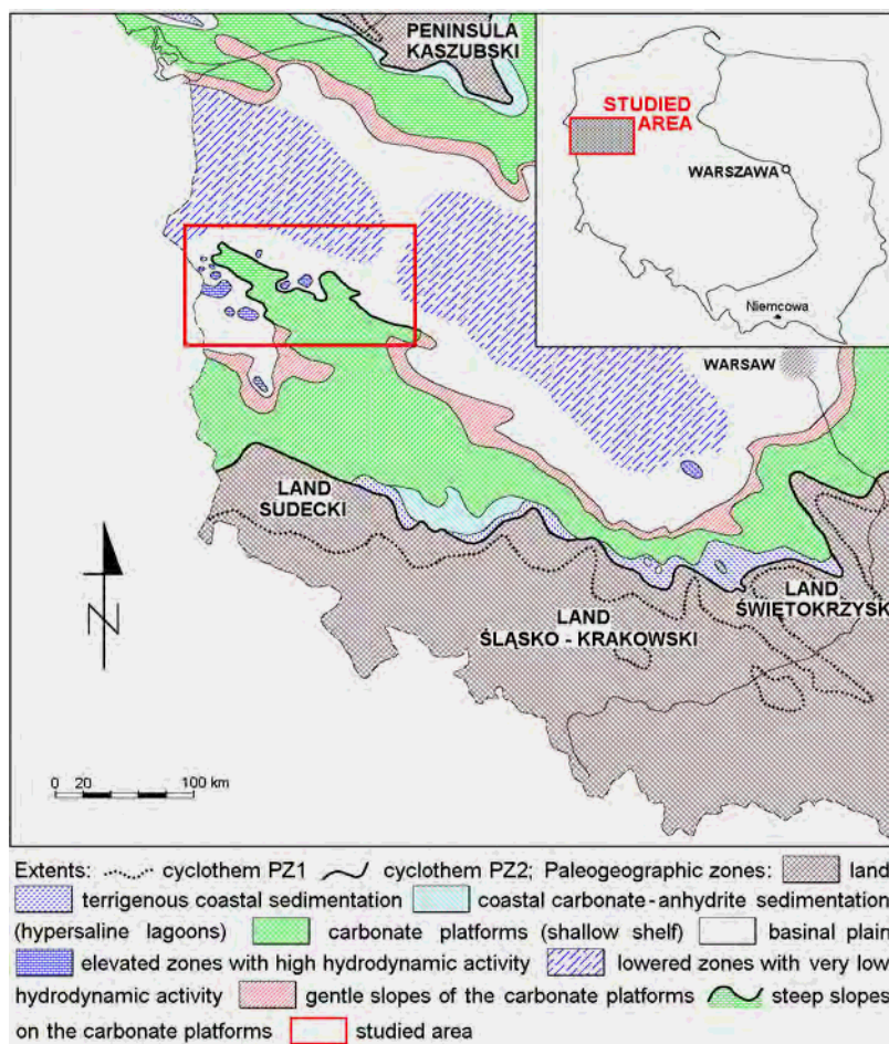
Fig. 1 Paleogeography of the Main Dolomite in the eastern part of the European Basin (R. Wagner - 1994, modified)
