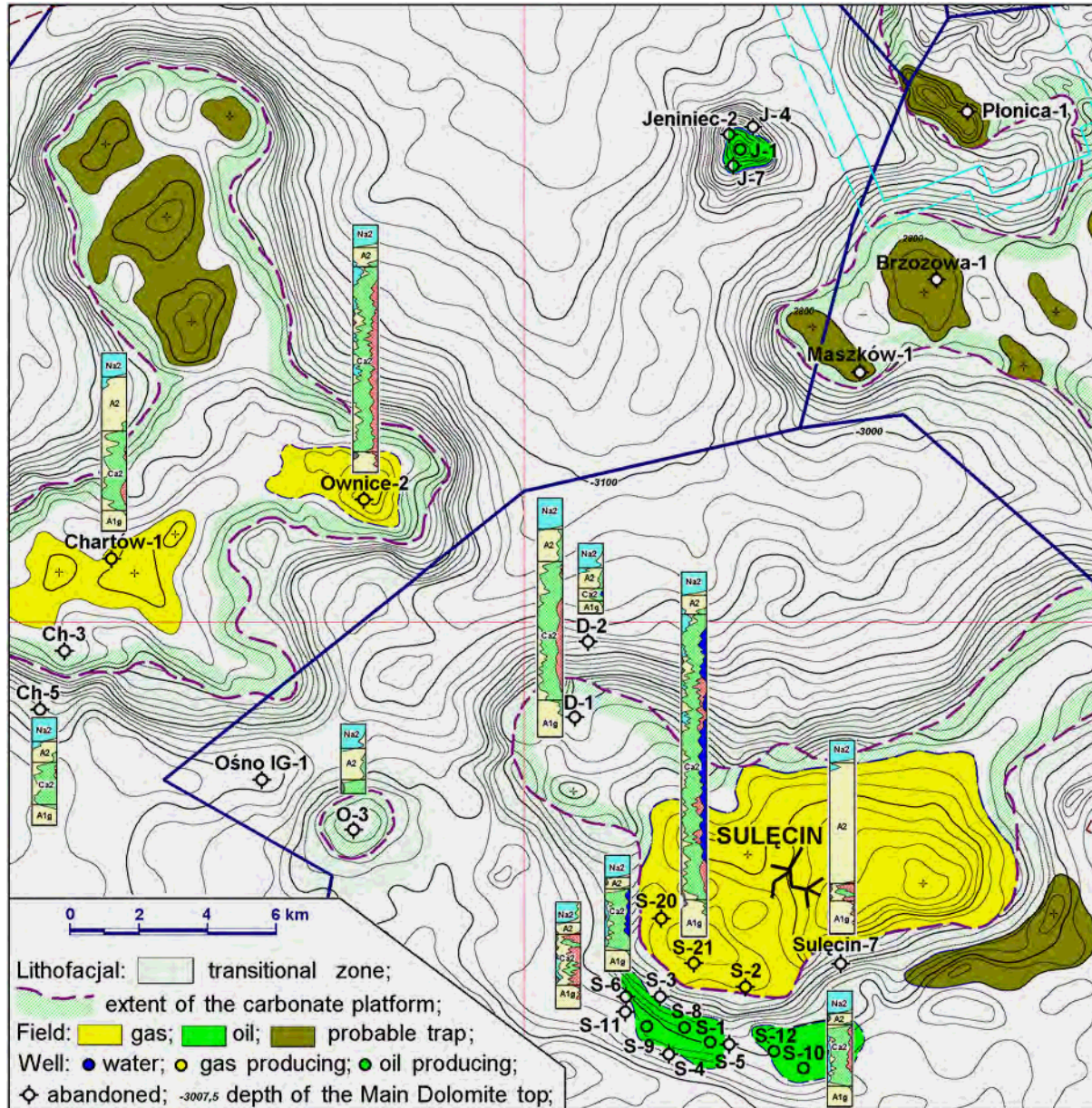
Fig. 2 Structural map in the area of Chartow - Sulecin - Jeniniec fields
