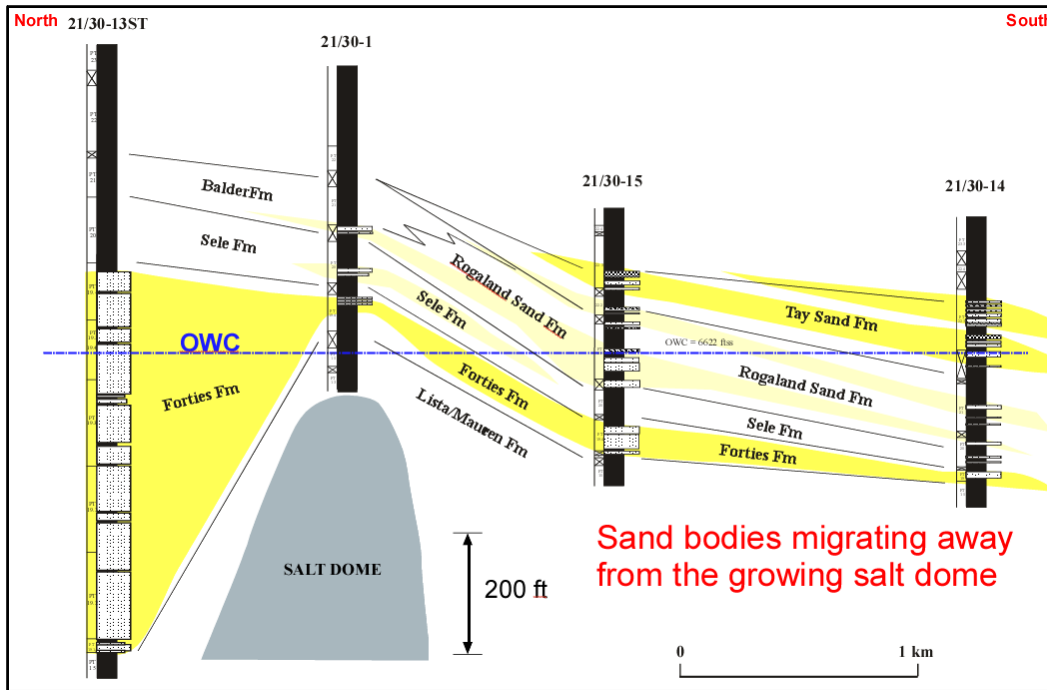
Fig. 3 North-South cross-section through the Gannet F Field
