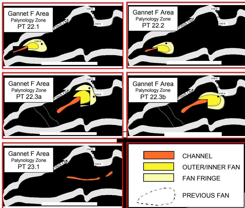
Fig. 4 Successive turbidite lobes filling a valley controlled by active salt tectonics
