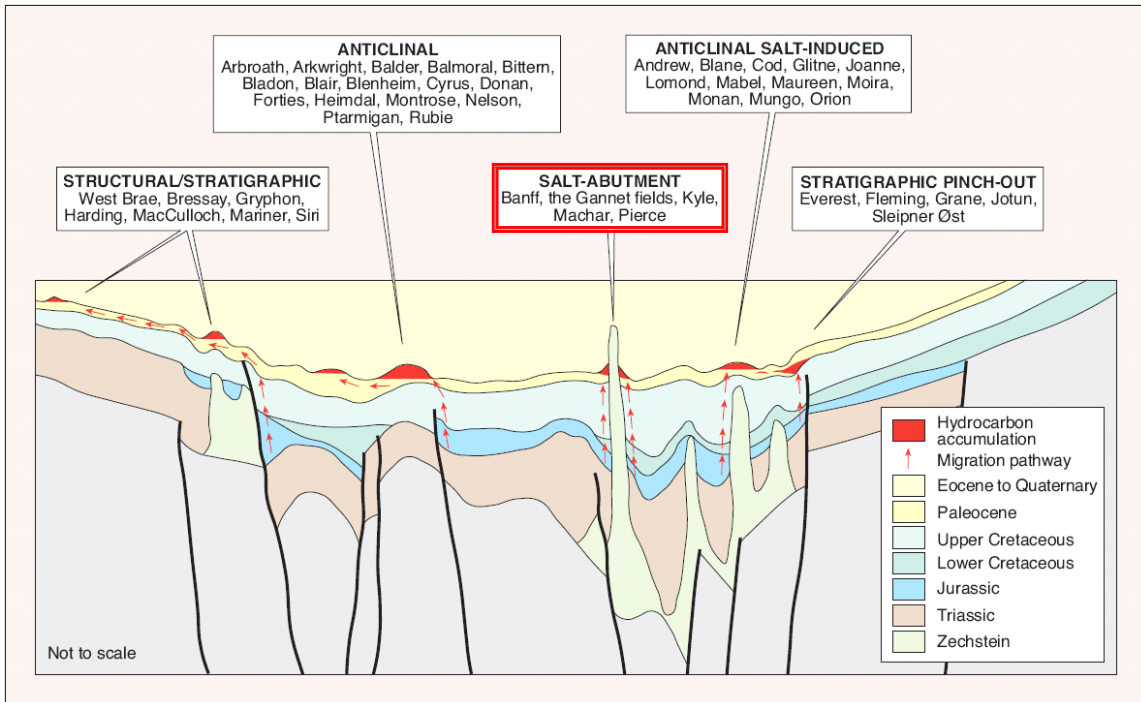
Fig. 1 Schematic representation of North Sea turbidite plays, after Ahmadi et al. 2003
