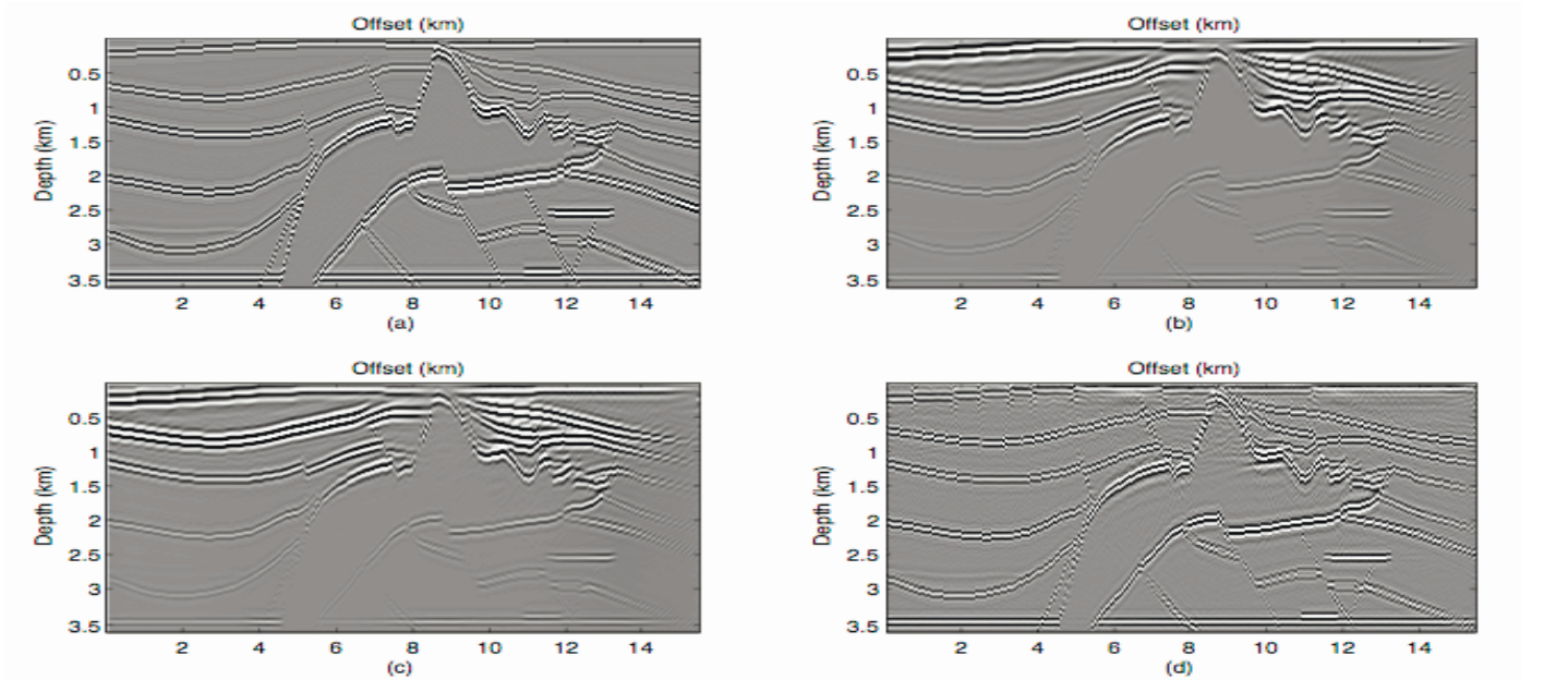
Figure 2. Amplitude recovery using eigenvalue decomposition of the normal operator, (a) SEG-AA' reflectivity model, (b) action of normal operator on (a), (c) action of approximated normal operator on (a), (d) amplitude recovered image applying the inverse of approximated normal operator on (b)
