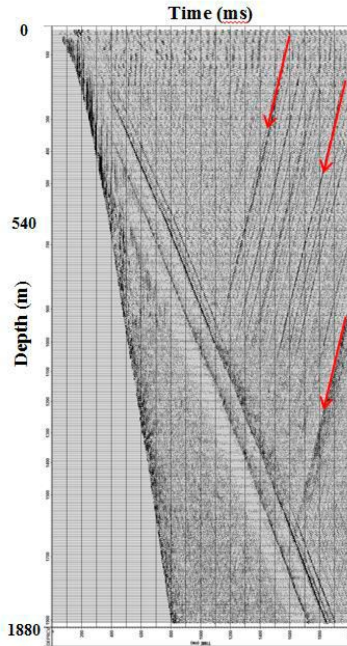
Figure 4. Processed zero-offset VSP data. Three of the interpreted upward tube waves are indicated by the red arrows.
