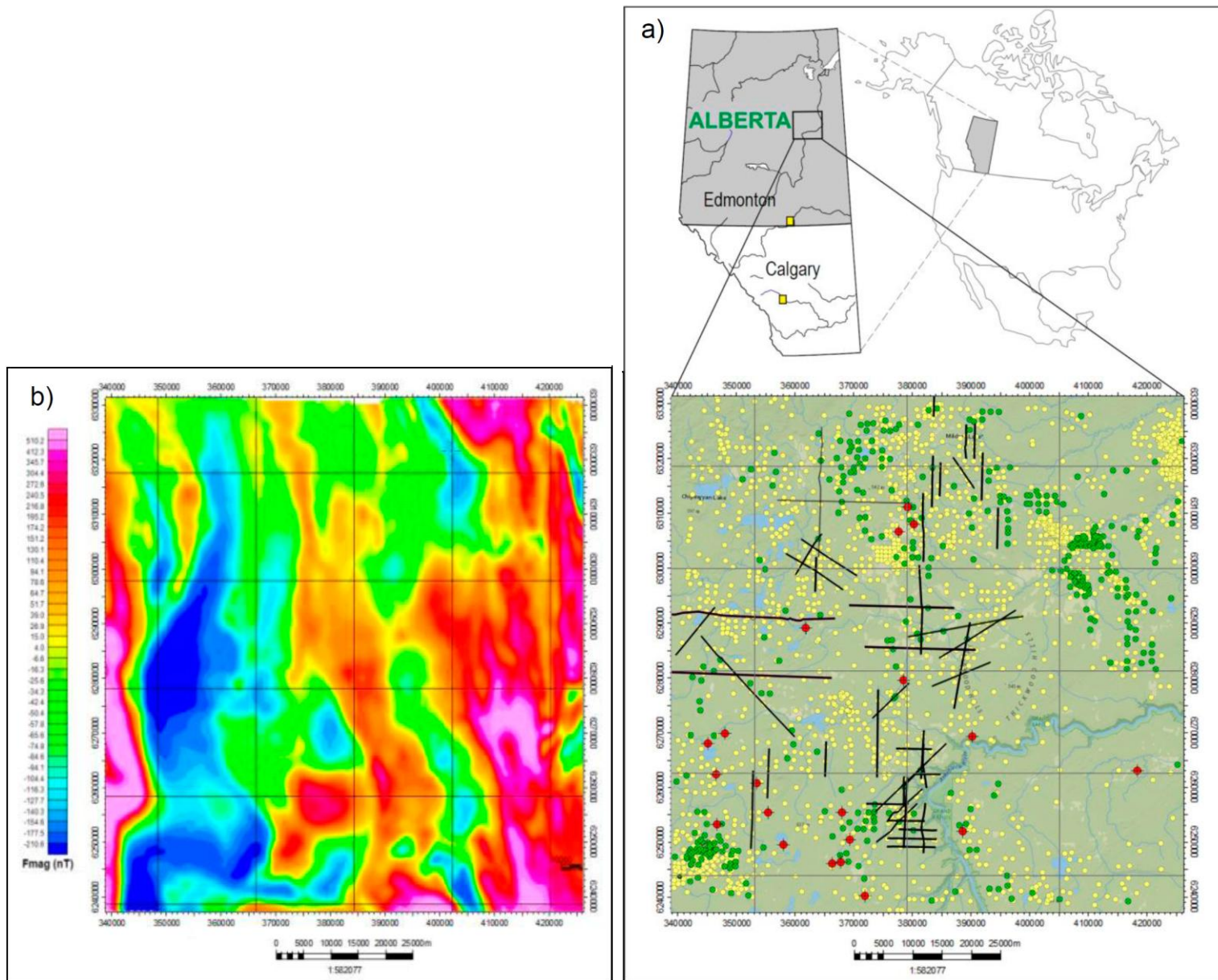
Figure 1. (a) The 2D profile (solid lines) and borehole (circles) locations in the study region. Darker colored circles are the boreholes drilled deeper than 500 m and contain Digital Sonic (DT) and Density (RHOB) in their log datasets. (b) Map of final total magnetic field after applying diurnal, leveling and cultural corrections.
