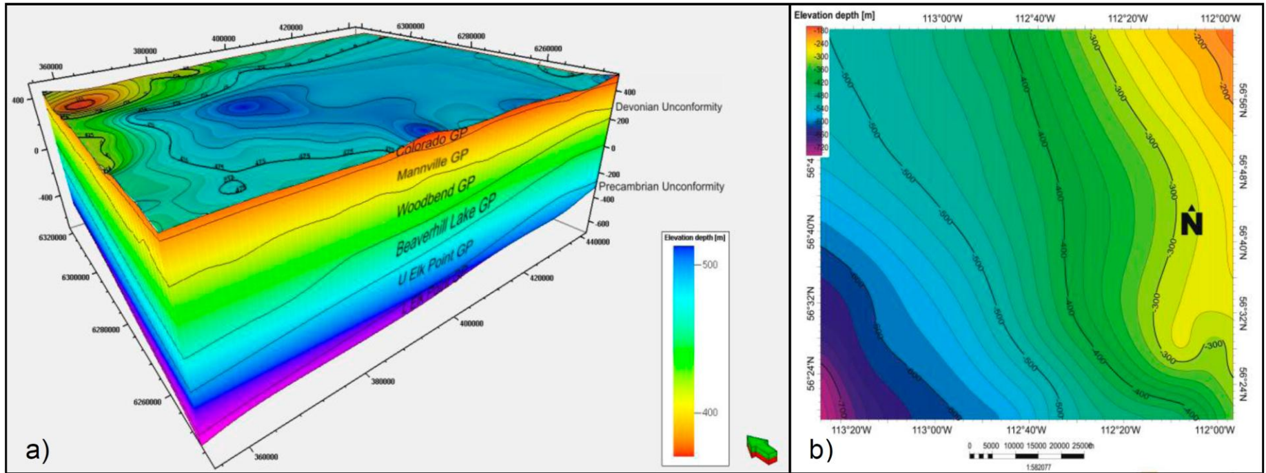
Figure 2. (a) 3D geological model in the study region in elevation depth domain. The axes units are in UTM-NAD83-Zone12 projection system. (b) The seismic-corrected Precambrian unconformity surface in the study area in elevation depth domain.
