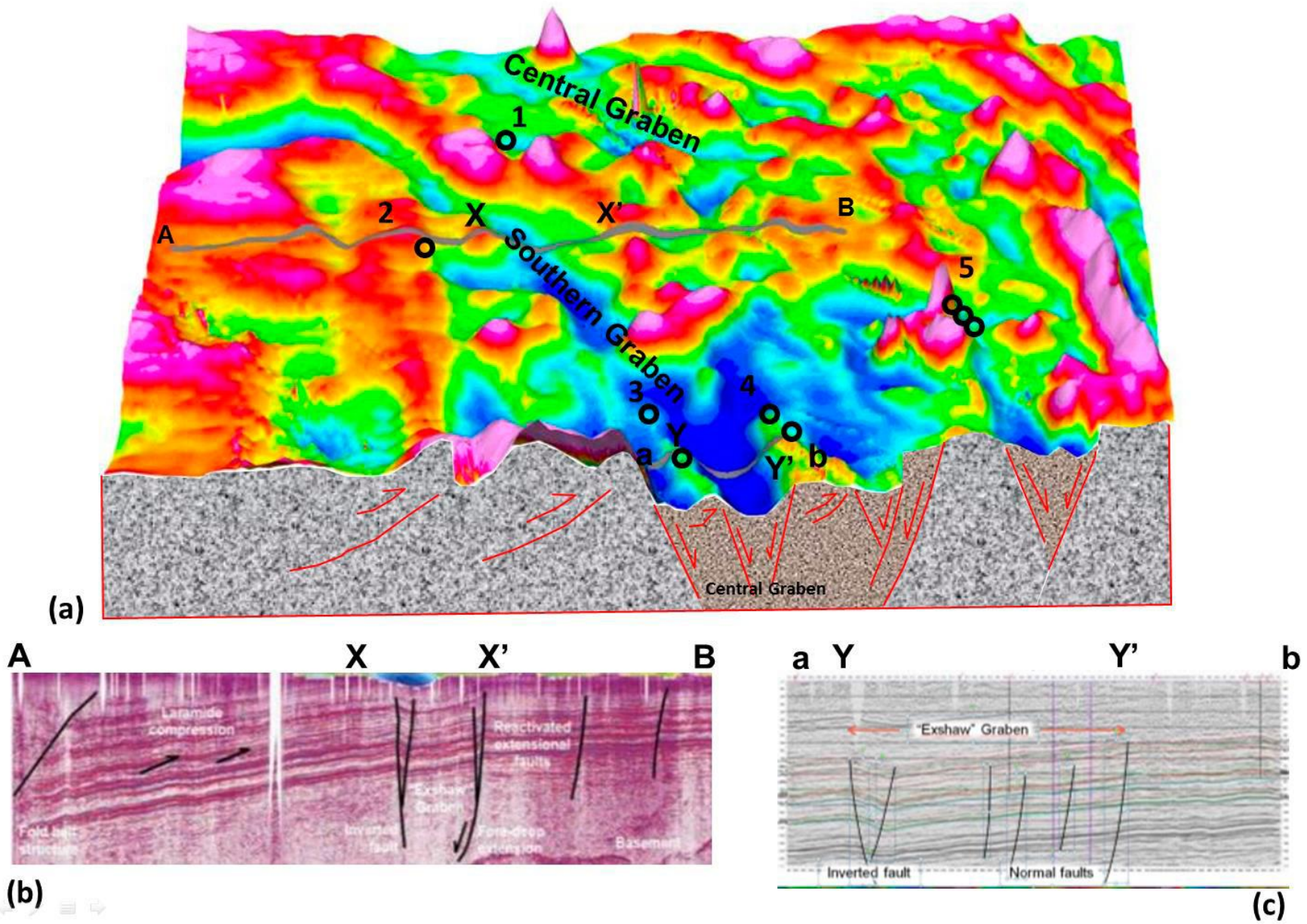
Figure 3. Three-dimensional diagram of High Resolution Magnetic data and regional seismic over the Canadian portion of the Exshaw/Big Valley play area. The circles represent Exshaw-Big Valley wells that produced over 250 bbl/d.
