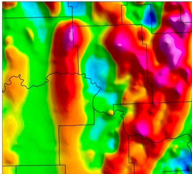
(c) Magnetic anomaly data
