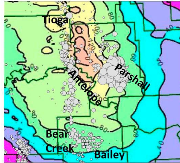
(b) Bakken isopach
