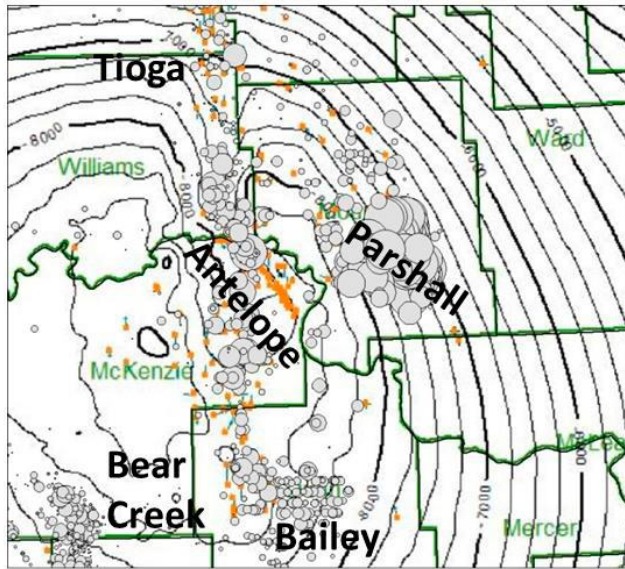
(a) Three Forks Structures
