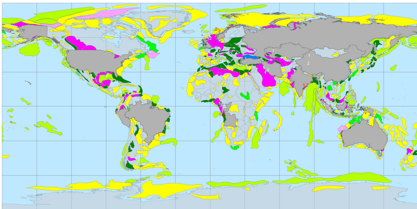
Figure 1. Global map of sedimentary provinces, from St. John et al. (1984), with overlay of countries (in gray) that had 2005 discoveries summarized in this article.
