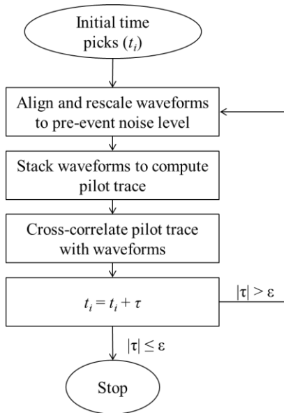
Figure 1: Iterative cross-correlation based workflow for refined arrival time picking by De Meersman et al. (2009).
