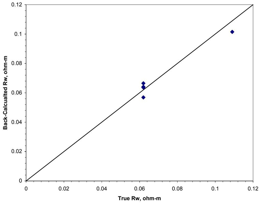
Figure 1. Comparison of back-calculated Rw and true Rw
