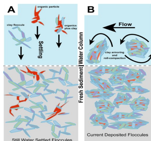
Figure 5: (at left) Contrasting sediment fabrics due to the difference between (A) simple settling and (B) accretion of mud bed from flow deposited floccules carried in bedload.
