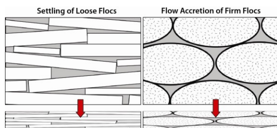
Figure 7: (at left) The impact of loose floccule settling and rolling-floc accretion on likely pore sizes and rock properties. Compacting (red arrows, bottom) and already parallel aligned loose floc deposit will likely produce abundant tiny pores in the 10's of nm range, whereas compaction of a layer of bedload floccules potentially allows preservation of pores in the micron range.
