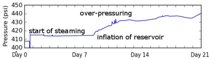
Figure 3. Pressure curve for a 21 day period.
