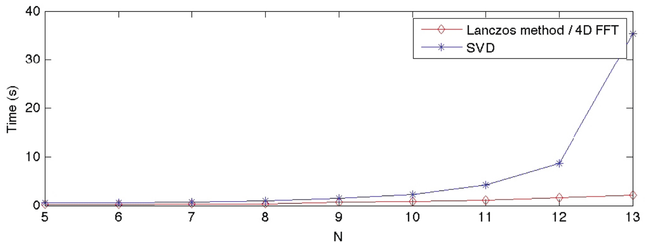
Figure 2. Evaluation of computational times of rank reduction. The survey consists of N x N x N x N traces, 512 samples, sampling rate is 2ms. The 4D cube was embedded in a Toeplitz matrix that was reduced to a rank k=5 matrix via the SVDS algorithm (Matlab) and the proposed Lanczos algorithms with fast matrix times vector multiplication via 4D FFTs.
