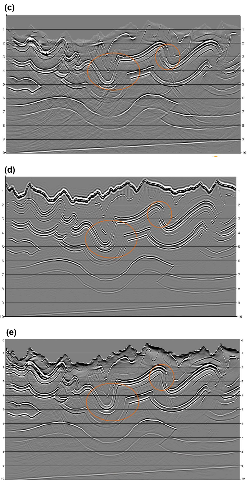
Figure 1. Depth migrated images from the Foothills model dataset. (a) Velocity model using for generating the synthetic data. (b) Reverse-time migration. (c) Kirchhoff migration. (d) Wave-equation migration. (e) Complex-beam migration.
