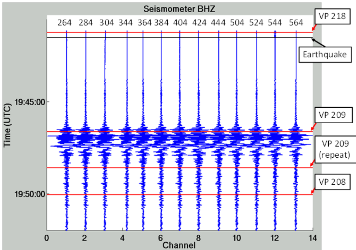
Figure 1: Vertical component of uncorrelated data from seismometers. Trace length is 11.5 minutes. The time of the first sweep (of two sweeps per vibe point) is shown as a red line. The time of the earthquake is shown as a black line.
