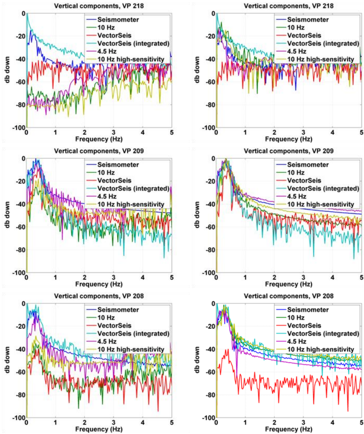
Figure 3: The first five Hertz of amplitude spectra for uncorrelated data from VP 218 (top; before earthquake arrivals), VP 209 (middle) and VP 208 (bottom), before correcting for geophone response (left column) and after correcting for geophone response (right).
