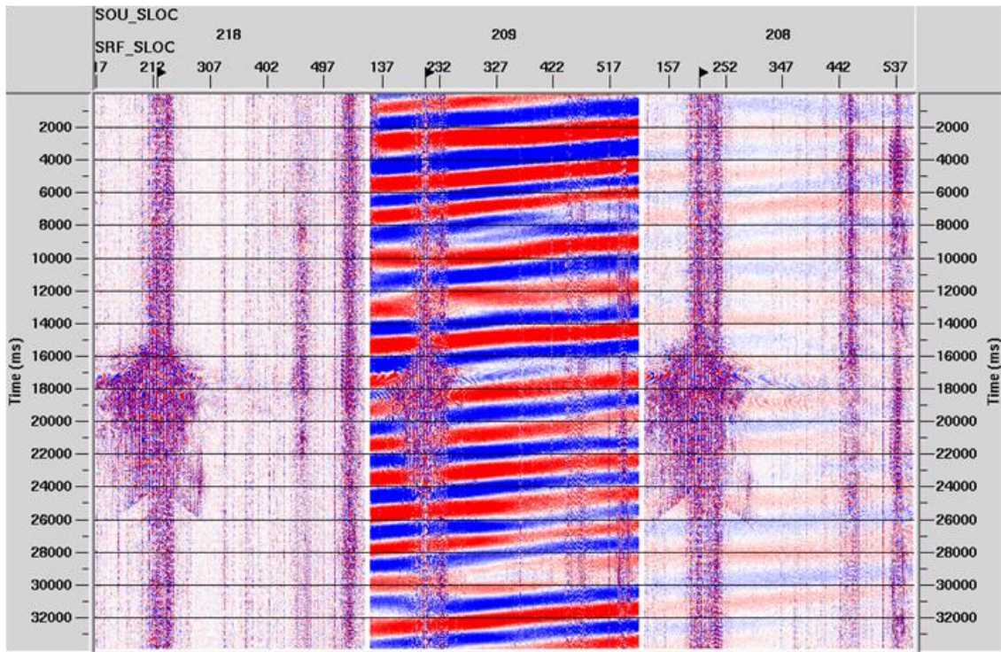
Figure 2: Uncorrelated data from the vertical component of VectorSeis accelerometers for VP 218 (left), VP 209 (middle), and VP 208 (right). Each source gather is 4.5 km wide. Trace length is 34 seconds, vertical fold is two. The Vancouver Island earthquake epicenter is ~1050 km to the right.
