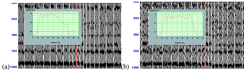
Figure 4. Seismic gathers shown (average spectra -inset) around a well location in CDP domain. Gathers (a) without spectral balancing (b) with spectral balancing. Ensemble based spectral balancing was done on data in (b) in common-offset domain. The red line indicates the location of the well.
