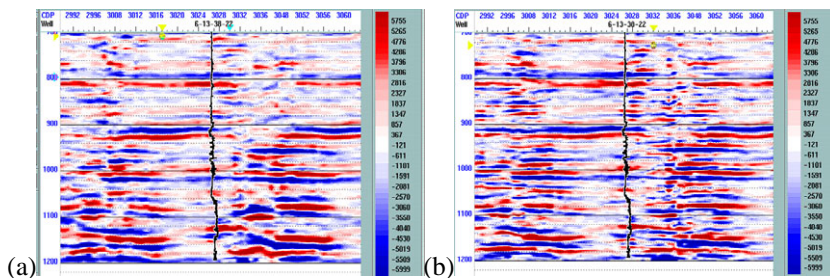
Figure 5. S-impedance reflectivity computed at well 1 location (a) section without spectral balancing (b) section with spectral balancing. Improved resolution and detail in gradient section resulted in improved S-impedance reflectivity using spectral balancing. The measured intercept, gradient responses matched the response predicted from logs at Viking, and Joli Fou horizons (880 ms and 912 ms).
