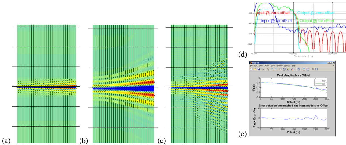
Figure 2. Synthetic model with Class 3 AVO anomaly (a) without stretch (reference model) (b) with stretch (same AVO as model without stretch) caused by move-out correction (c) after moveout correction and spectral balancing, (d) amplitude spectra of stretched model before and after spectral balancing. The colored spectra are marked by text in the same color. In Figure 2e, the measured amplitude vs offset at trough of the event is shown. The top panel in Figure 2e shows the amplitude vs offset plot for reference (blue) and spectral balanced gathers (green). The bottom panel in Figure 2e shows the error between reference and spectral balanced output at the trough of the event. From the error plot, it can be seen that for most offsets, the error is less than 10%.
