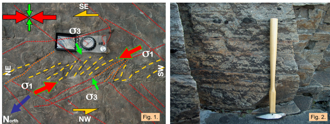
Figure 1, left: Mapview along strike of dm wide simple shear zone (sinistral / Riedel, yellow), striking as the bisectrix of the conjugate set of subvertical shear fractures (red). At least one of the conjugate sets abuts against the sinistral shear zone.
