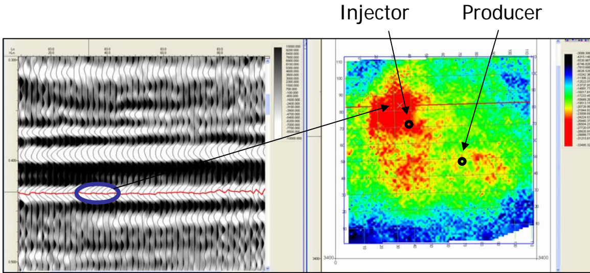
Figure3: Vertical component data. On the left is the pick of the target coal event. On the right is the amplitude map of the picked event. The line displayed on the left is the east-west (inline) line just north of the injector well. The blue circle on the left highlights the high amplitude anomaly that is shown by the red colour on the right hand side.
