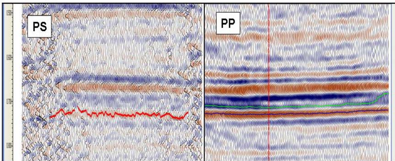
Figure 5: Comparison of the PS data (left) which has been stacked into an E-W 2D line and the comparable PP data (right) at the well location (red line). The Arbour/Mynheer Coal event is picked in red on the PS section.
