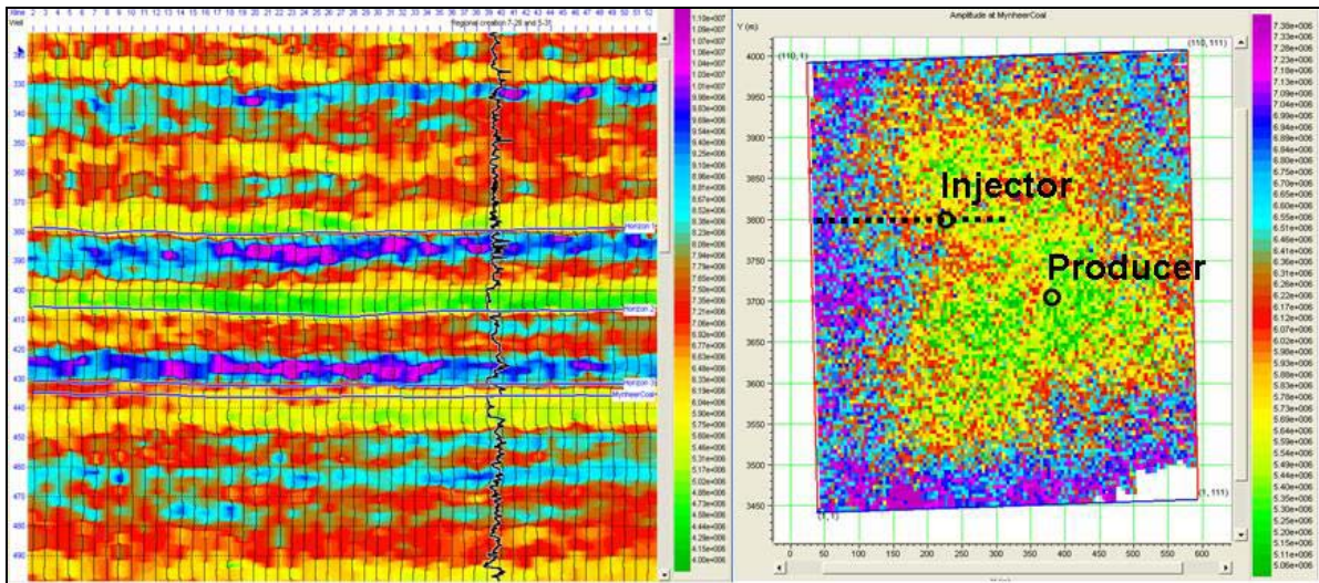
Figure 4: Acoustic impedance section and horizon impedance slice at the Mynheer seismic event. The density log is imposed over the section. Note that the dynamic range is not the same between the two images.
