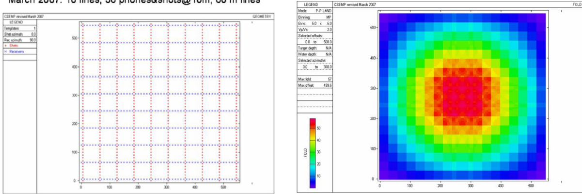
Figure 2: On the left is the layout design for the vertical component 3D baseline 3D survey. Receiver lines run east-west and source lines run north-south. On the right is the expected fold for the PP survey
