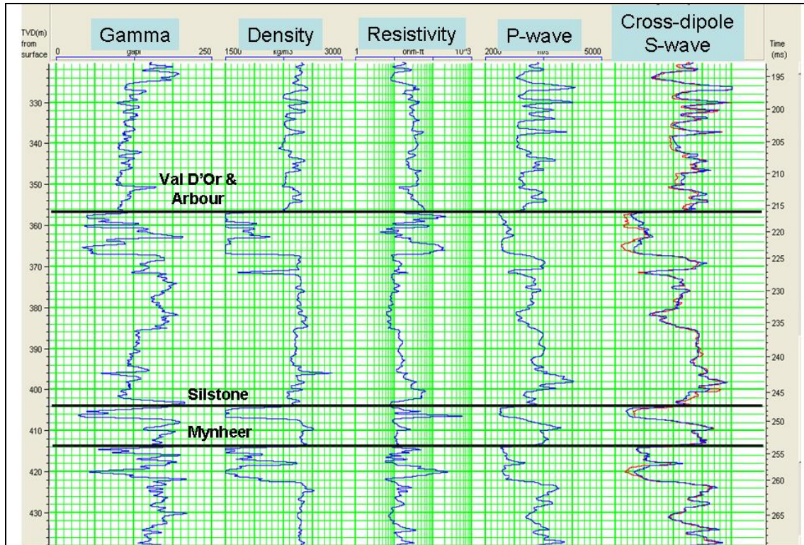
Figure1: Petrophysical logs from the injection well showing the Ardley Coal Zone
