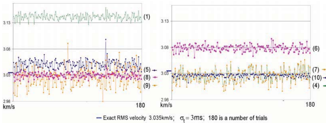
Figure 3. RMS velocity estimations through different NMO approximations in the presence of random noise
